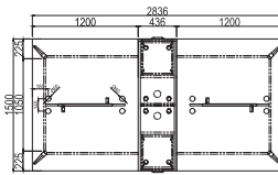
WORKSTATION CLUSTER OF 4 C/W FILING CABINET & WOODEN HANGING DIVIDER PANEL
