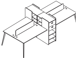
WORKSTATION CLUSTER OF 4 C/W FILING CABINET & WOODEN HANGING DIVIDER PANEL
