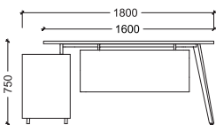
Front View (Visitor Side)
