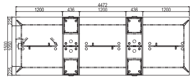
WORKSTATION CLUSTER OF 6 C/W FILING CABINET & WOODEN HANGING DIVIDER PANEL
