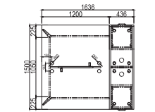
WORKSTATION CLUSTER OF 2 C/W FILING CABINET & WOODEN HANGING DIVIDER PANEL
