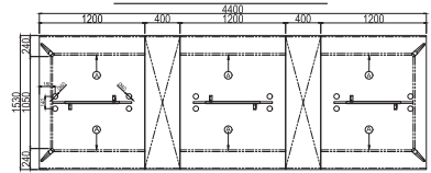
WORKSTATION SET - CLUSTER OF 6 C/W FIXED PEDESTAL 2D2F
