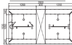
WORKSTATION SET - CLUSTER OF 4 C/W FIXED PEDESTAL 2D2F
