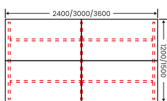
ML LEG CONCEPT - 4 PAX FACE TO FACE
