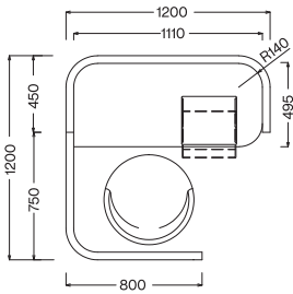
SIZE : (L) 1200 mm * (W) 1200 mm * (HT) 1350 mm
