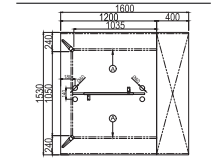
WORKSTATION SET - CLUSTER OF 2 C/W FIXED PEDESTAL 2D2F
